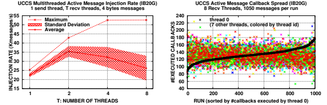
Figure 2: Injection rate and load fairness for Active Message communications with multiple receiver threads.
