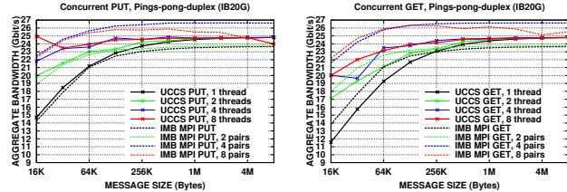
Figure 1: Aggregate bandwidth of one-sided communication primitives, issued by multiple threads concurrently.
